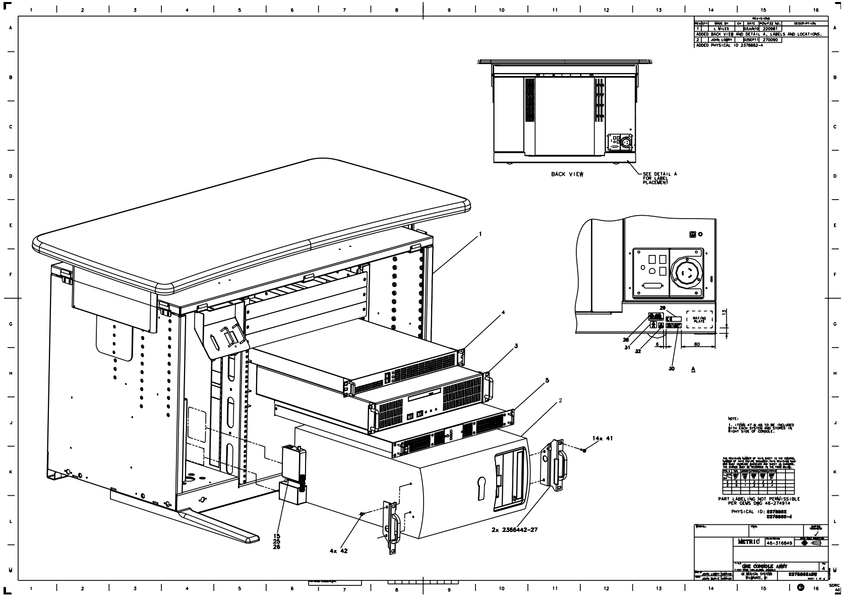
Figure 2: GRE Console (2378862, sheet 1, rev 04)
