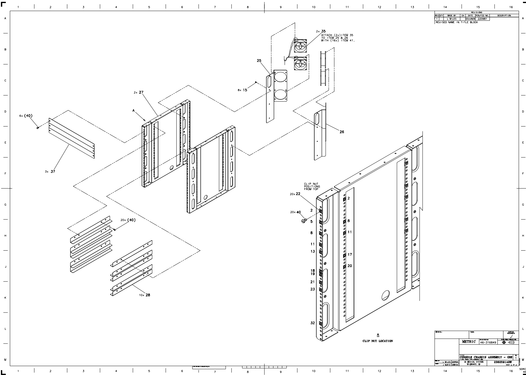
Figure 6: Console Chassis Assembly (2362591 sheet 2, rev 1)
