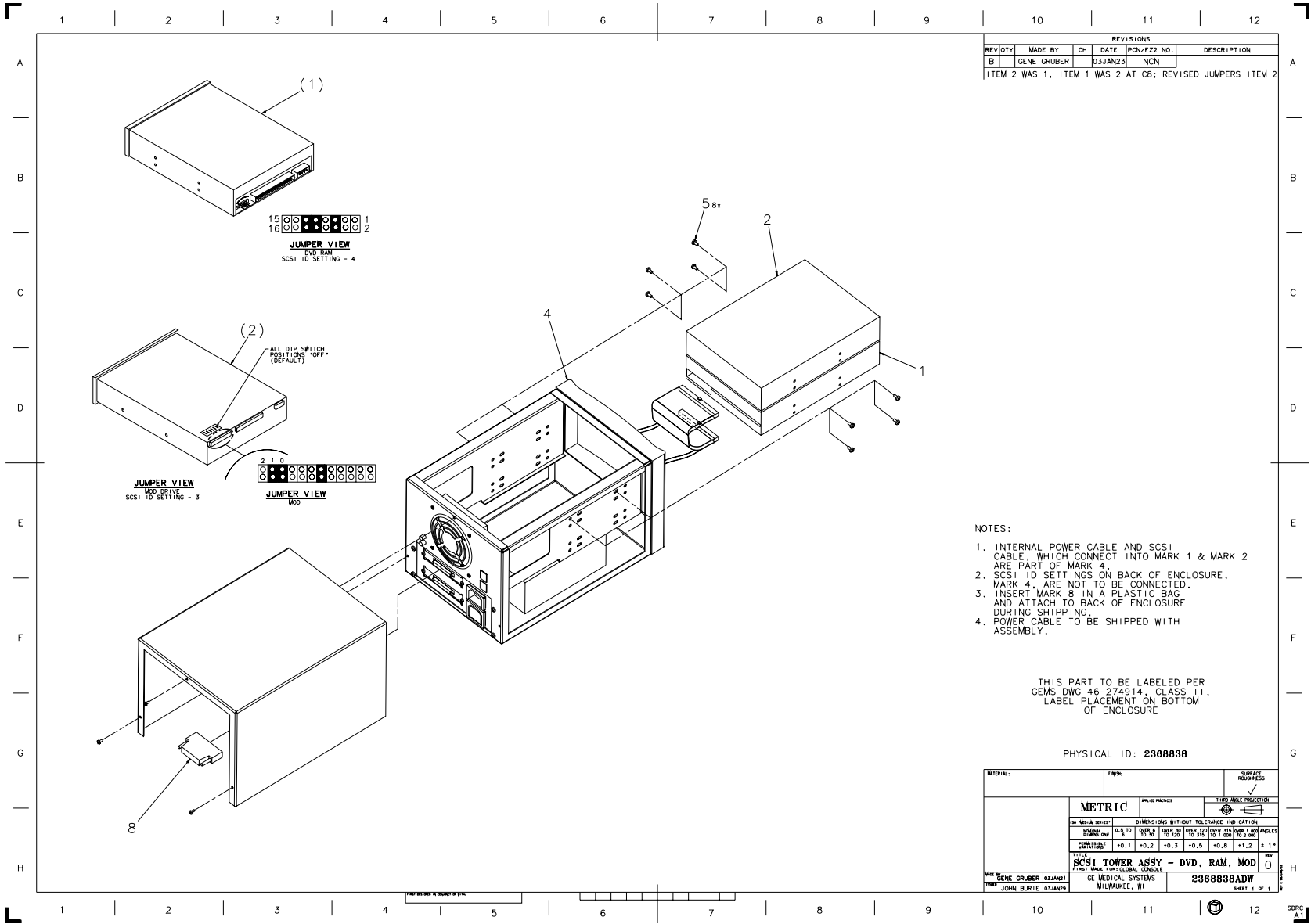
Figure 9: SCSI Tower, DVD-RAM, MOD (2368838, sheet 1, rev 0)
