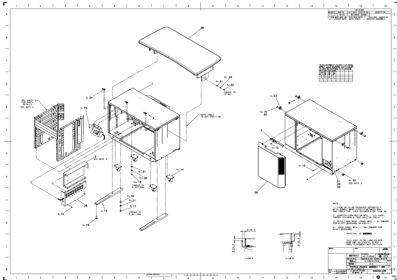
Figure 5: Console Chassis Assembly (2362591 sheet 1, rev 1)
